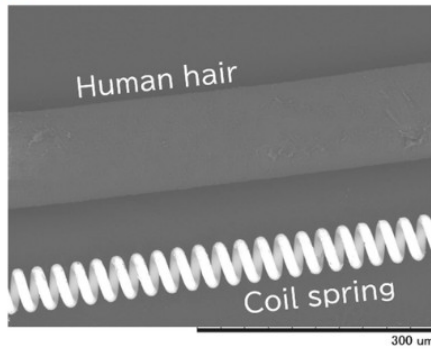
Ultra-fine spring with a wire diameter of 13 \mu m and an outer diameter of 53 \mu m
