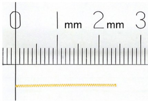
Ultra-fine spring with a wire diameter of 13 \mu m and an outer diameter of 53 \mu m
